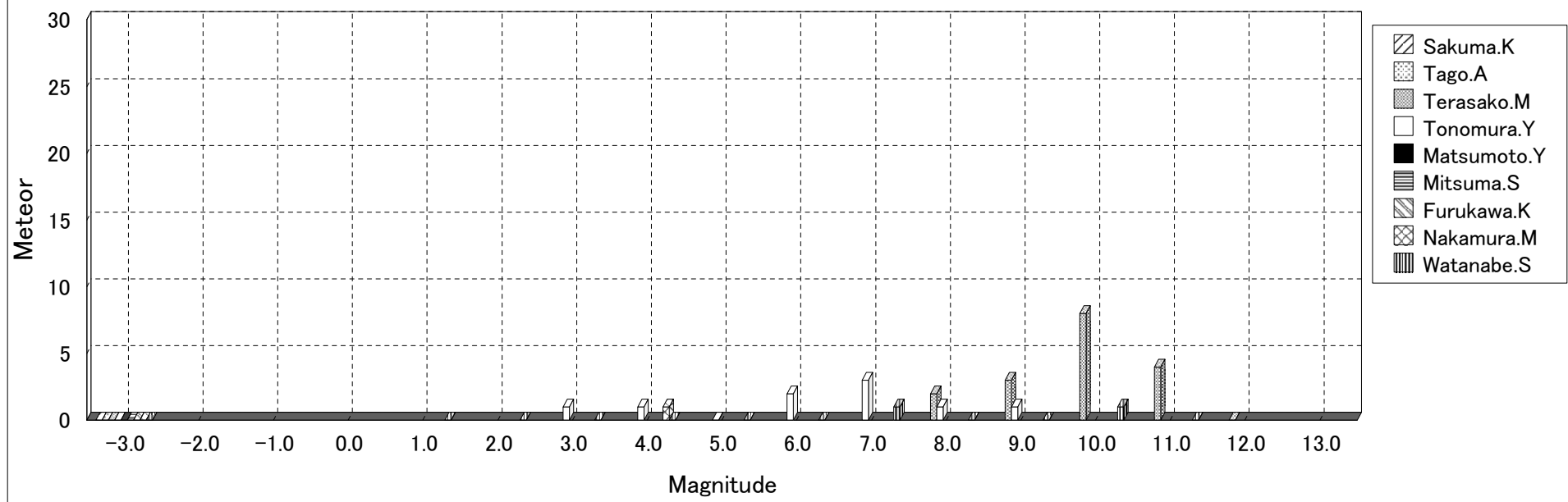
Magnitude Distributions of the Telescopic observations in February,2001
