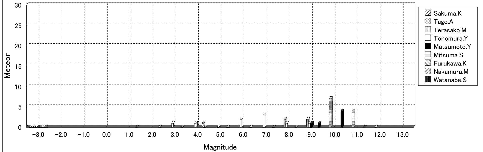
Magnitude Distributions of the Telescopic observations in March,2001
