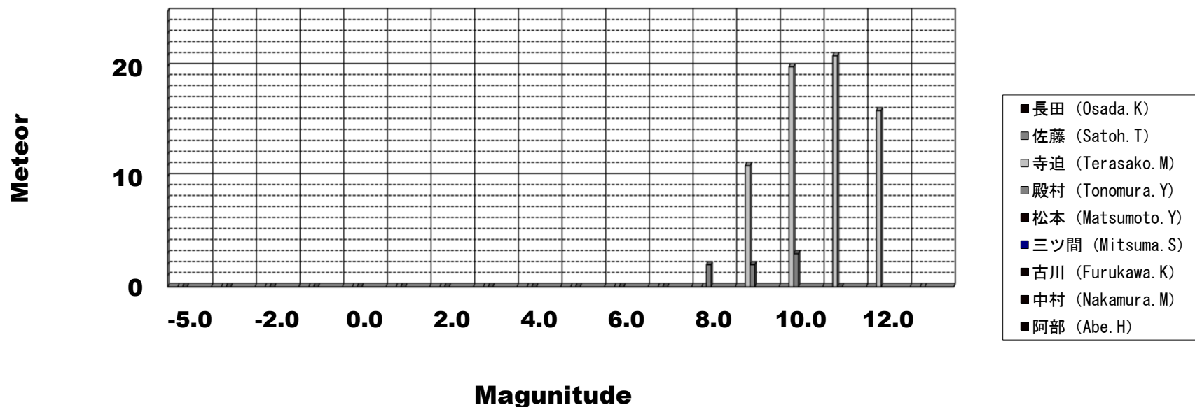
Magnitude Distributions of the Telescopic observations in November,2020
