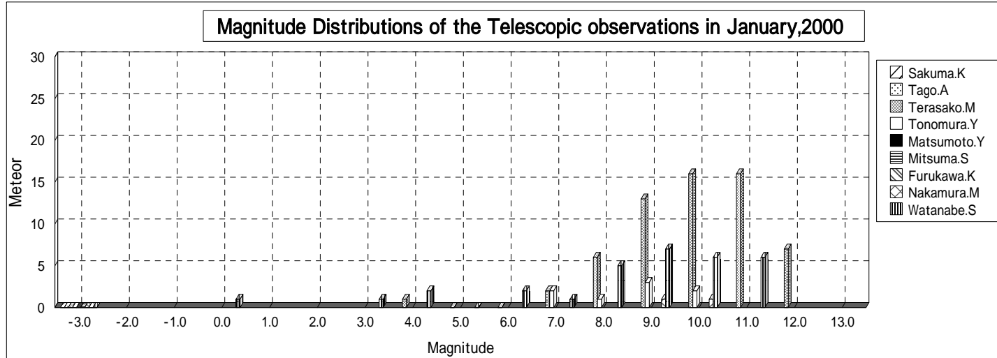
Magnitude Distributions of the Telescopic observations by Terasako
